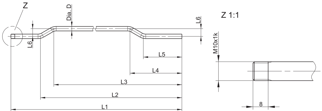
Pic. 2: with thread, at FAZ03954-10 and FAZ03954-11
