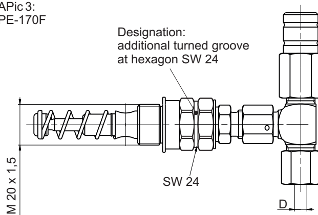
Pic. 4: Pipe connection dia. 8:
