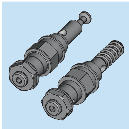
Pic. 1: PE-120 V for electric Pump EP-1
